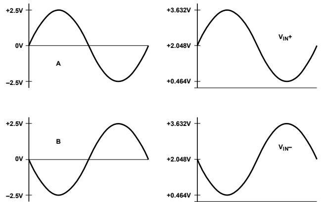
Figure 35. Differential Amplifier Signal Conditioning
