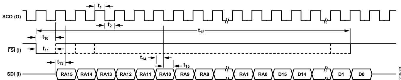
Figure 3. AD7764 Register Write
