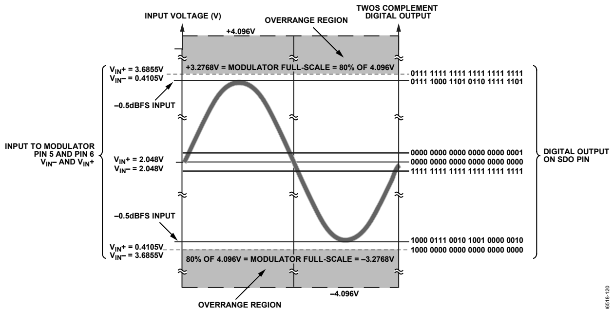
Figure 33. AD7764 Scaling: Modulator Input Voltage vs. Digital Output Code
