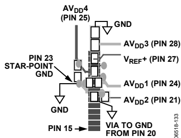
Figure 46. Supply Decoupling
