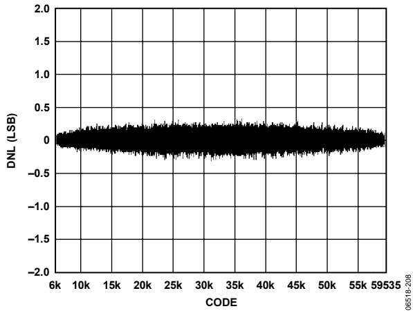
Figure 24. DNL Plot
