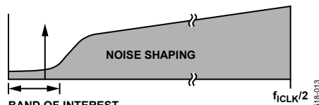
Figure 30. \Sigma - \Delta ADC, Noise Shaping
