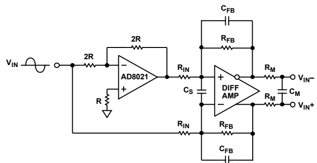
Figure 36. Single-Ended-to-Differential Conversion
