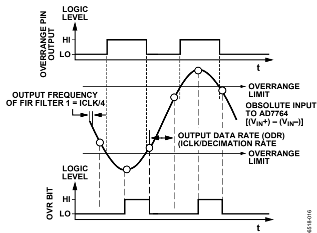
Figure 38. \overline{\text{OVERRANGE}} Pin and OVR Bit vs. Absolute Voltage Applied to Modulator
