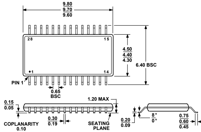
COMPLIANT TO JEDEC STANDARDS MO-153-AE Figure 49. 28-Lead Thin Shrink Small Outline [TSSOP] (RU-28) Dimensions shown in millimeters
